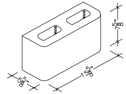
6" X 8" X 16" HOLLOW DOUBLE BULLNOSE (ALSO IN 18")
