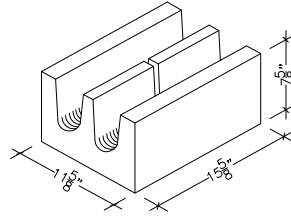
12" X 8" X 16" SOLID BOTTOM BOND BEAM (ALSO IN 18")
