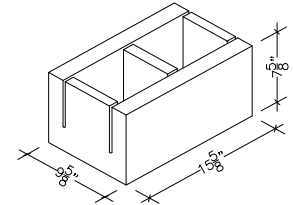
10" X 8" X 16" OPEN BOTTOM BOND BEAM (ALSO IN 18")
