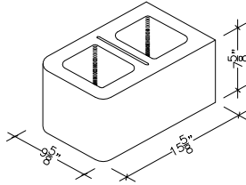
10" X 8" X 16" HOLLOW SINGLE BULLNOSE PIER (ALSO IN 18")
