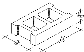
HALF HIGH 10" X 4" X 16" HOLLOW STRETCHER (ALSO IN 18")
