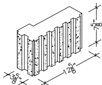
4" X 8" X 13" SOLID CORNER SPLIT RIB
