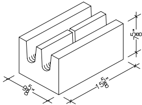
10" X 8" X 16" SOLID BOTTOM BOND BEAM (ALSO IN 18")
