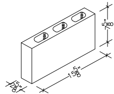
3" X 8" X 16" HOLLOW (ALSO IN 18")
