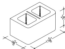
10" X 8" X 16" HOLLOW DOUBLE BULLNOSE PIER
