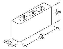
4" X 8" X 16" HOLLOW SINGLE BULLNOSE CORNER (ALSO IN 18")
