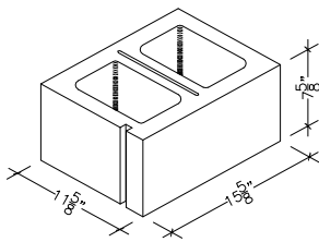
12" X 8" X 16" HOLLOW CORNER SASH (ALSO IN 18")
