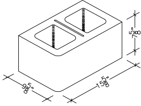
10" X 8" X 16" HOLLOW SINGLE BULLNOSE CORNER (ALSO IN 18")
