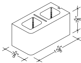
8" X 8" X 16" HOLLOW SINGLE BULLNOSE CORNER SASH (ALSO IN 18")
