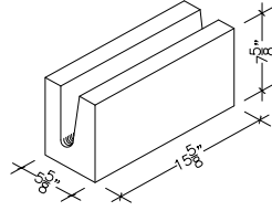
6" X 8" X 16" BOND BEAM LINTEL (ALSO IN 18")
