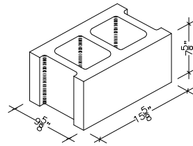
10" X 8" X 16" HOLLOW STRETCHER (ALSO IN 18")
