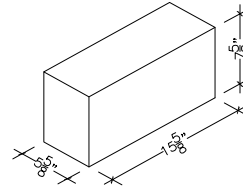
6" X 8" X 16" SOLID
