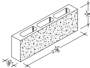
4" X 8" X 24" HOLLOW SPLIT FACE
