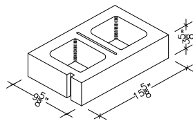
HALF HIGH 10" X 4" X 16" HOLLOW CORNER SASH (ALSO IN 18")
