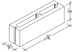
6" X 8" X 24" HOLLOW DOUBLE CORNER SASH
