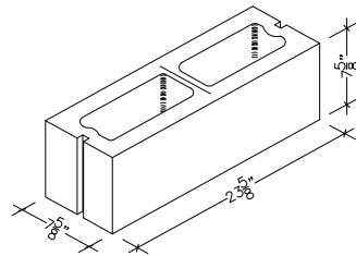
8" X 8" X 24" HOLLOW DOUBLE CORNER SASH
