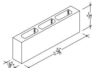
4" X 8" X 24" HOLLOW
