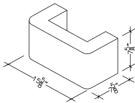
8" X 8" X 16" COLUMN COVER
