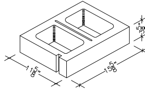
HALF HIGH 12" X 4" X 16" HOLLOW CORNER SASH (ALSO IN 18")
