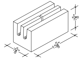
8" X 8" X 16" SOLID BOTTOM BOND BEAM (ALSO IN 18")
