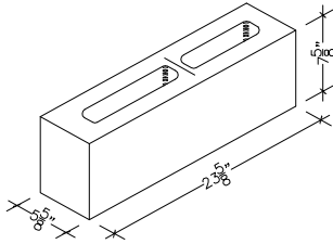
6" X 8" X 24" HOLLOW STRETCHER
