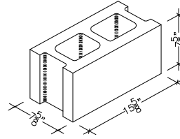
8" X 8" X 16" HOLLOW STRETCHER (ALSO IN 18")
