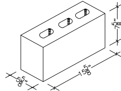
6" X 8" X 16" 75% SOLID (ALSO IN 18")
