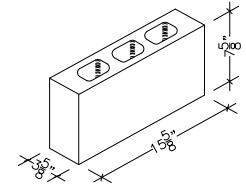
4" X 8" X 16" HOLLOW (ALSO IN 18")
