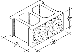
12" X 8" X 16" HOLLOW STRETCHER SPLIT FACE (ALSO IN 18")
