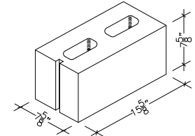
8" X 8" X 16" 75% SOLID CORNER SASH (ALSO IN 18")
