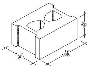
12" X 8" X 16" 75% SOLID (ALSO IN 18")
