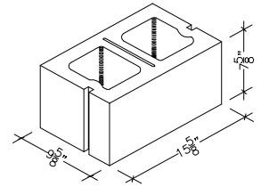
10" X 8" X 16" HOLLOW DOUBLE CORNER SASH (ALSO IN 18")
