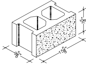
10" X 8" X 16" HOLLOW STRETCHER SPLIT FACE (ALSO IN 18")
