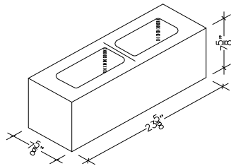
8" X 8" X 24" HOLLOW STRETCHER
