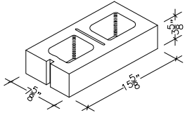
HALF HIGH 8" X 4" X 16" HOLLOW CORNER SASH (ALSO IN 18")
