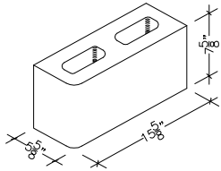
6" X 8" X 16" HOLLOW SINGLE BULLNOSE CORNER (ALSO IN 18")
