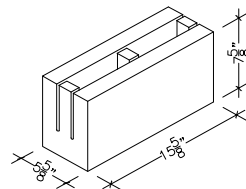
6" X 8" X 16" OPEN BOTTOM BOND BEAM (ALSO IN 18")
