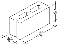
6" X 8" X 16" HOLLOW CORNER SHASH (ALSO IN 18")
