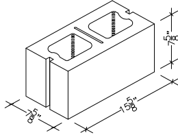
8" X 8" X 16" HOLLOW DOUBLE CORNER SASH (ALSO IN 18")
