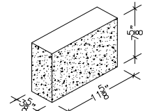
4" X 8" X 12" CORNER SPLIT FACE
