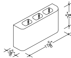
4" X 8" X 16" HOLLOW DOUBLE BULLNOSE PIER (ALSO IN 18")
