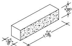
HALF HIGH 4" X 4" X 16" SPLIT FACE
