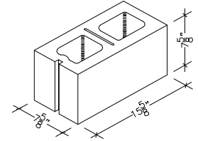
8" X 8" X 16" HOLLOW CORNER SASH (ALSO IN 18")
