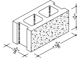
8" X 8" X 16" HOLLOW STRETCHER SPLIT FACE (ALSO IN 18")
