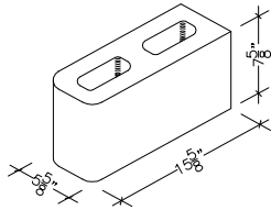
6" X 8" X 16" HOLLOW DOUBLE BULLNOSE CORNER (ALSO IN 18")
