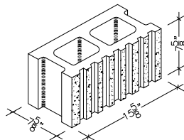
8" X 8" X 16" HOLLOW STRETCHER SPLIT RIB
