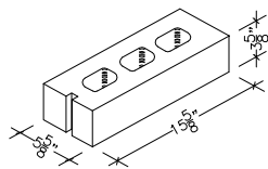
HALF HIGH 6" X 4" X 16" HOLLOW STRETCHER CORNER SHASH (ALSO IN 18")
