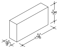
4" X 8" X 16" SOLID (ALSO IN 18")
