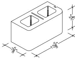
8" X 8" X 16" HOLLOW DOUBLE BULLNOSE (ALSO IN 18")
