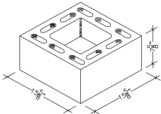
16" X 8" X 16" CHIMNEY BLOCK
