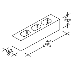
HALF HIGH 4" X 8" X 16" HOLLOW (ALSO IN 18")
