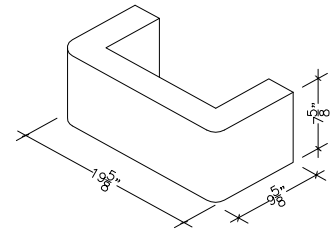
10" X 8" X 20" COLUMN COVER
