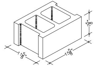
12" X 8" X 16" HOLLOW STRETCHER (ALSO IN 18")
