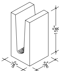
8" X 16" X 8" BOND BEAM LINTEL (ALSO IN 18")
