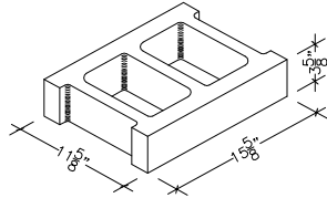
HALF HIGH 12" X 4" X 16" HOLLOW STRETCHER (ALSO IN 18")
