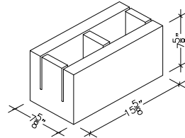
8" X 8" X 16" OPEN BOTTOM BOND BEAM (ALSO IN 18")
