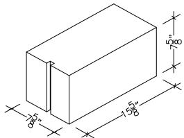
8" X 8" X 16" SOLID CORNER SASH
