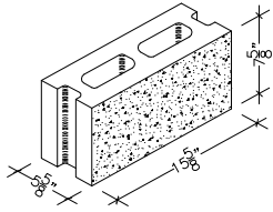
6" X 8" X 16" HOLLOW STRETCHER SPLIT FACE (ALSO IN 18")
