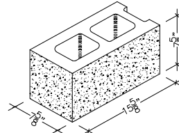
8" X 8" X 16" HOLLOW CORNER SPLIT FACE
