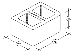
12" X 8" X 16" HOLLOW DOUBLE BULLNOSE (ALSO IN 18")
