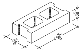
HALF HIGH 8" X 4" X 16" HOLLOW STRETCHER (ALSO IN 18")
