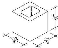
8" X 8" X 8" HOLLOW HALF BLOCK
