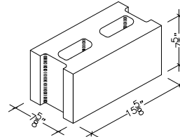
8" X 8" X 16" 75% SOLID (ALSO IN 18")
