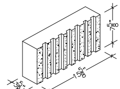
4" X 8" X 16" SOLID STRETCHER SPLIT RIB
