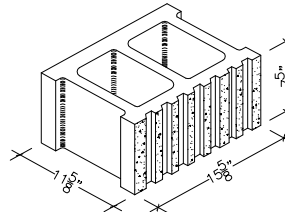
12" X 8" X 16" HOLLOW STRETCHER SPLIT RIB
