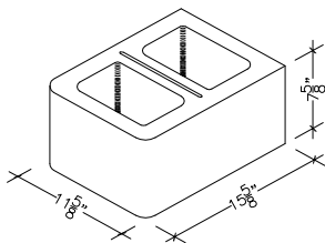
12" X 8" X 16" HOLLOW DOUBLE BULLNOSE (ALSO IN 18")
