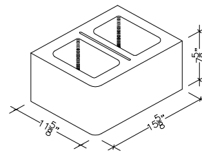
12" X 8" X 16" HOLLOW SINGLE BULLNOSE CORNER (ALSO IN 18")
