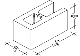
8" X 8" X 16" A SHAPED BLOCK (ALSO IN 18")
