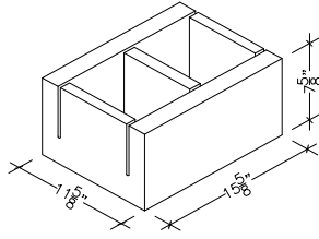
12" X 8" X 16" OPEN BOTTOM BOND BEAM (ALSO IN 18")
