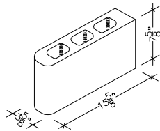
4" X 8" X 16" HOLLOW DOUBLE BULLNOSE CORNER (ALSO IN 18")
